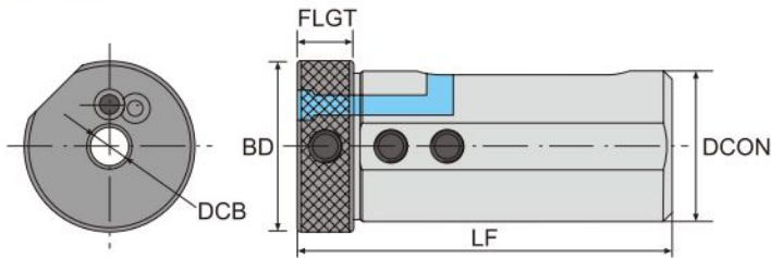
內徑出水套筒 Sleeve With Coolant Hole 材質：鋼 Shank：Steel
