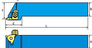
螺紋車刀架 Threading Tool Holder
