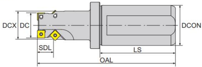
沉頭鑽 Countersunk Drill
