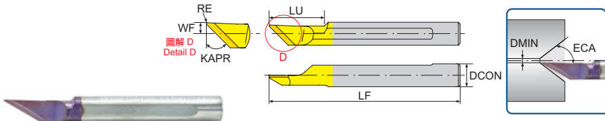
微小徑倒角及仿型鑄鋼內徑車刀 Tiny Chamfering & Profiling Carbide Boring Bar
