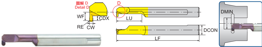
微小徑圓鼻開槽鎢鋼內徑車刀 Tiny Full Radius Grooving Carbide Boring Bar
