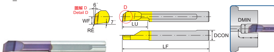
微小徑車削鎢鋼內徑車刀 Tiny Turning Carbide Boring Bar
