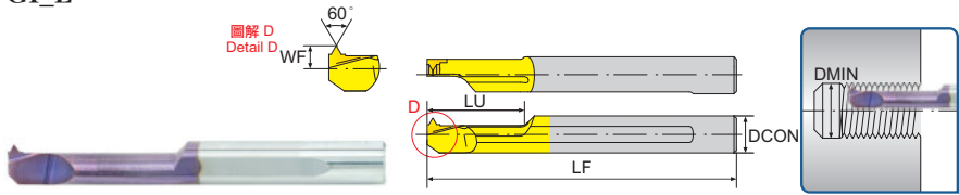
微小徑螺紋鎢鋼內徑車刀 Tiny Threading Carbide Boring Bar
