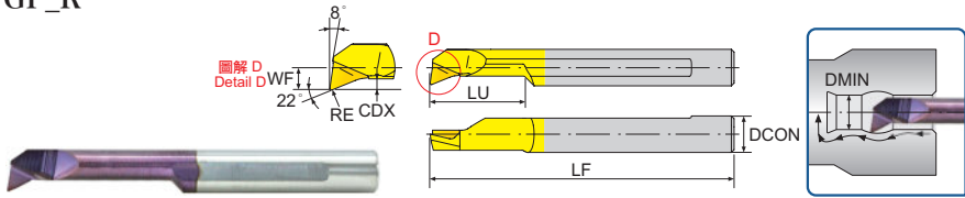
微小徑仿型車削鎢鋼內徑車刀 Tiny Profiling Carbide Boring Bar
