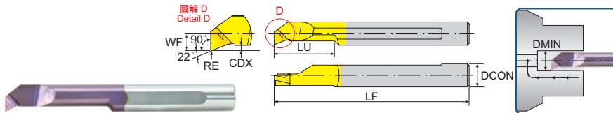
微小徑90°仿型鎢鋼內徑車刀 Tiny 90° Profiling Carbide Boring Bar
