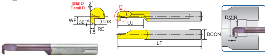
微小徑後掃車削鑄鋼內徑車刀 Tiny Bank Turning Carbide Boring Bar
