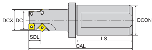
沉頭鑽 Countersunk Drill
